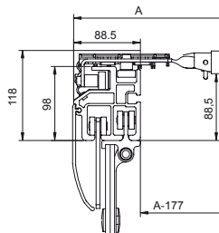
Profil MULTILINER Combi Profile MULTILINER Combi
