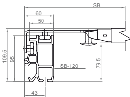
Profil SLIMLINER Small Profile SLIMLINER Small
