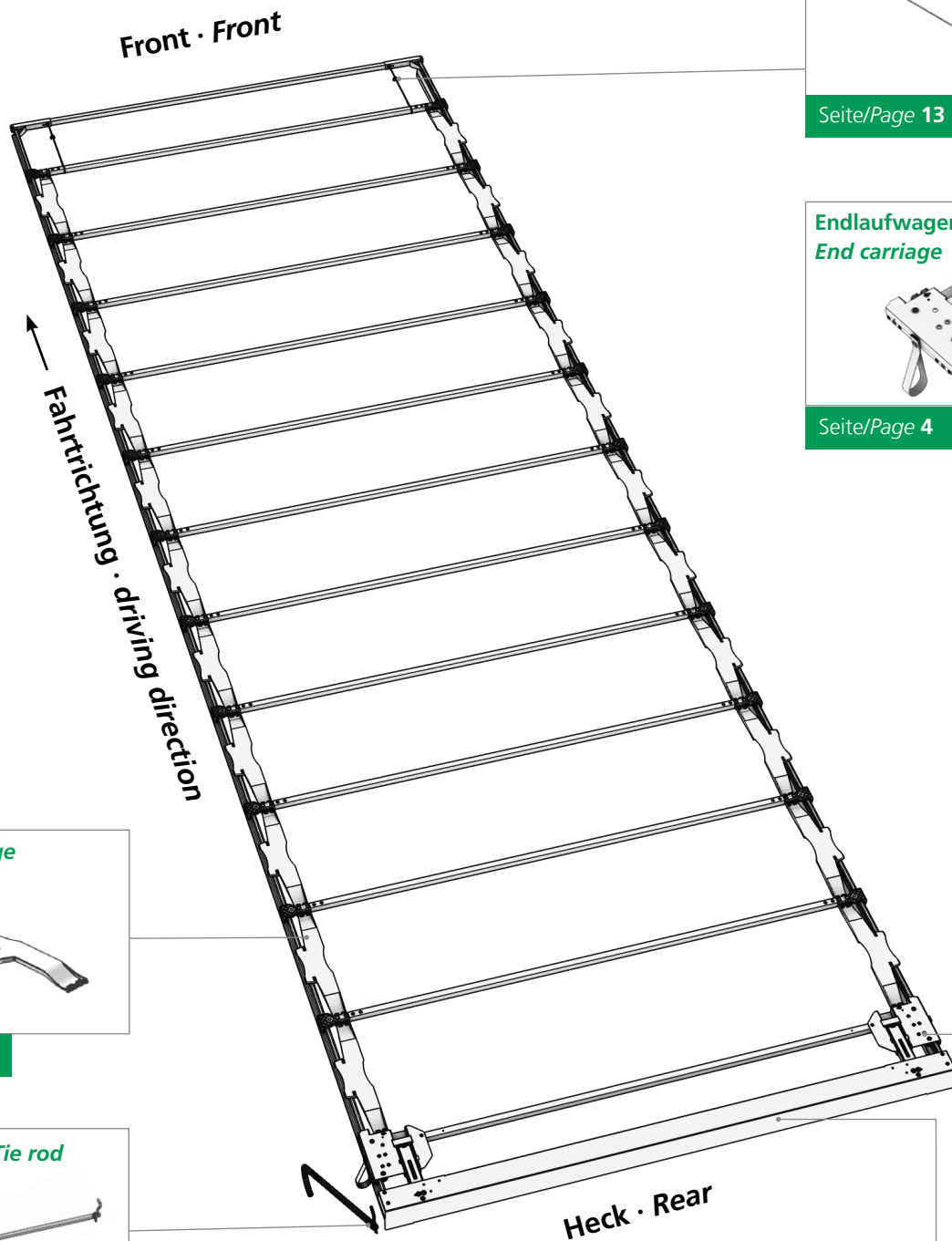
Portalbalken Gantry beam
